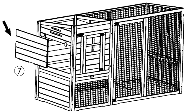
7. Insert the detachable door.
